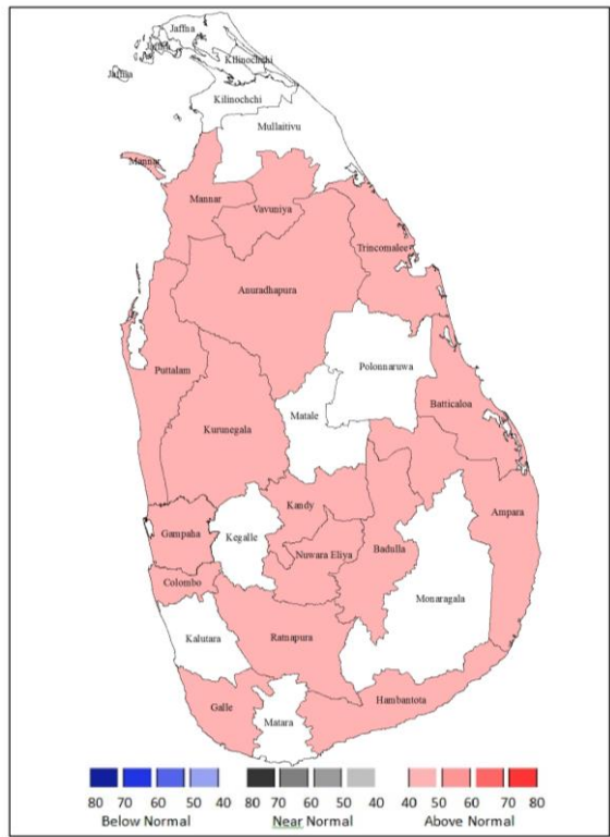
Fig 2: Probabilistic forecast for Minimum Temperatures for August 2019
