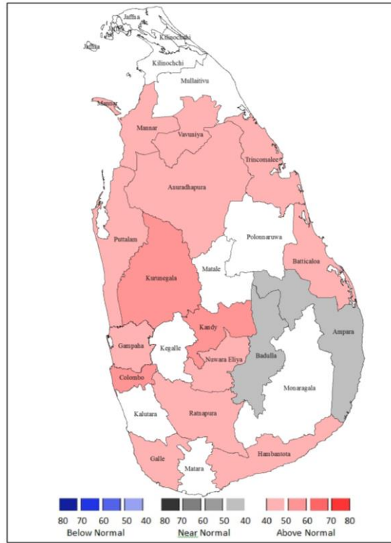
Fig 1: Probabilistic forecast for Maximum Temperatures for August 2019
