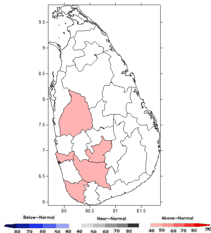
Fig 1: Probabilistic forecast for Maximum Temperatures for September 2019
