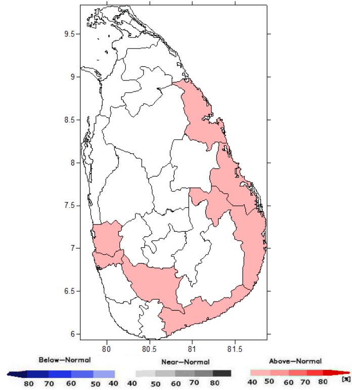
Fig 2: Probabilistic forecast for Minimum Temperatures for September 2019
