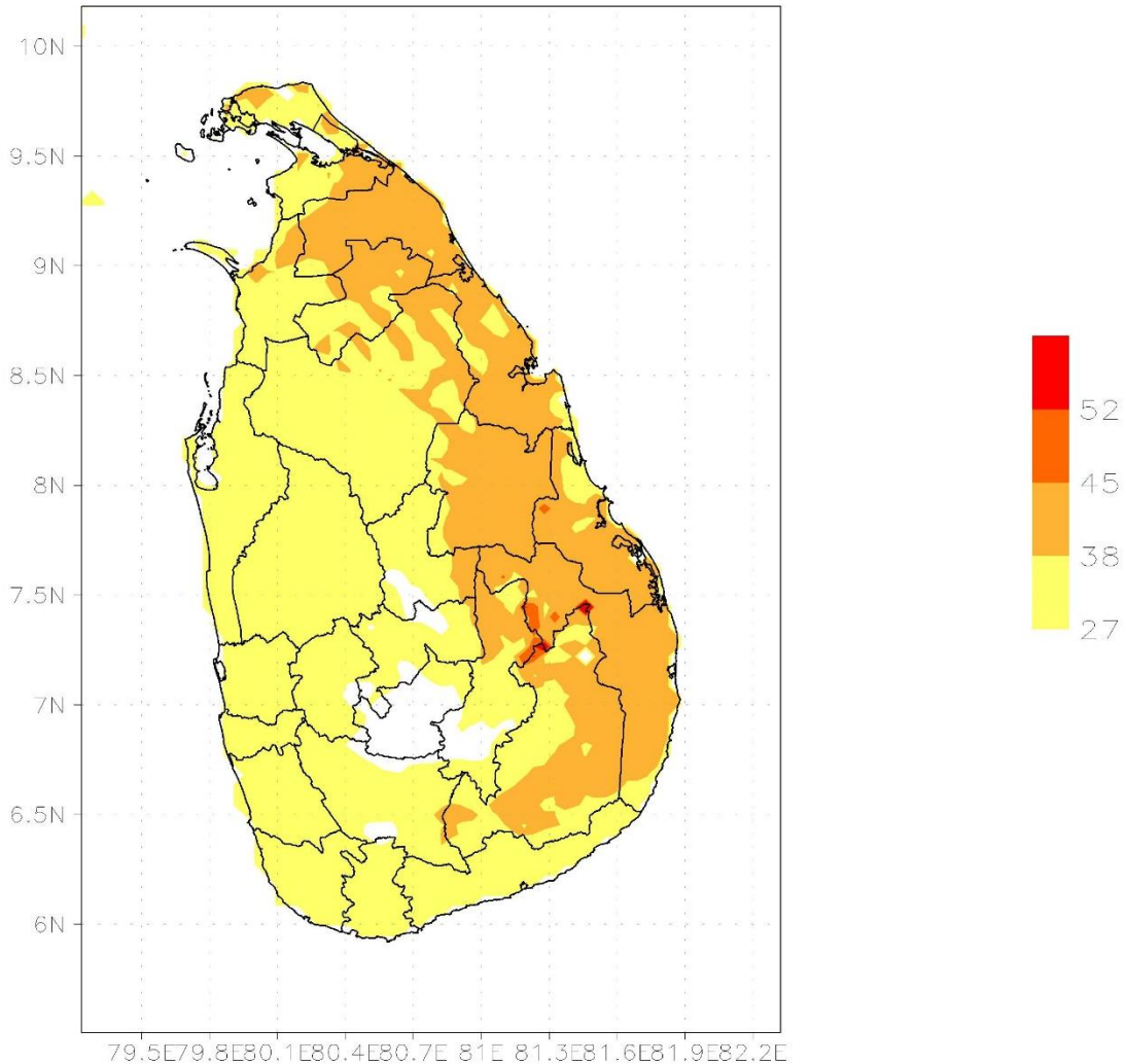
Heat Index WRFDA 5km 09UTC of 08/05/2018
